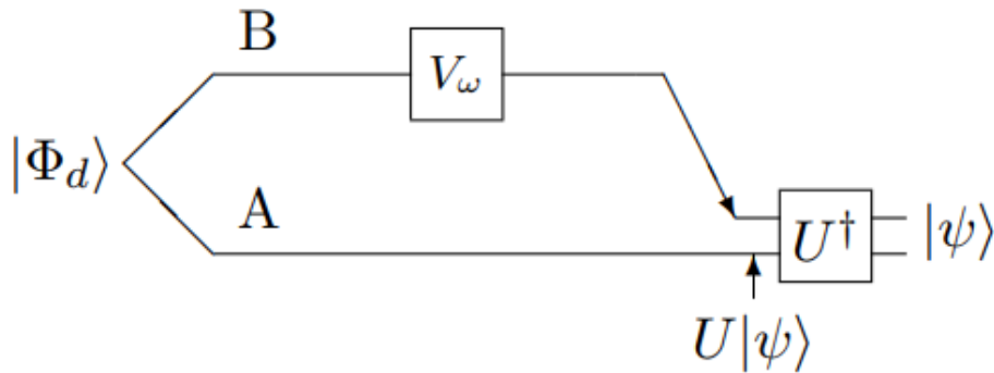
Figure 1.3: Superdense coding, image from [Hayden]
