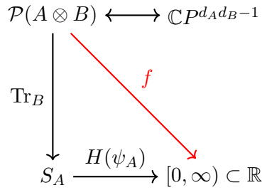
Figure 1.4: Mathematical structure for Hayden's concentration of measure phenomenon
